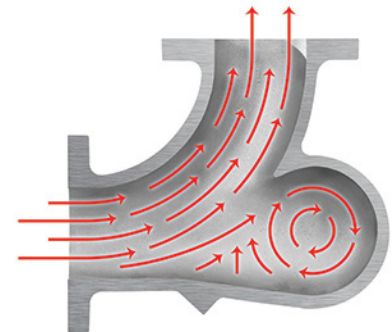
The Smart Elbow deflection elbow is available in a variety of materials and a wide range of pipe and tube sizes. For more information, contact HammerTek Corporation.
