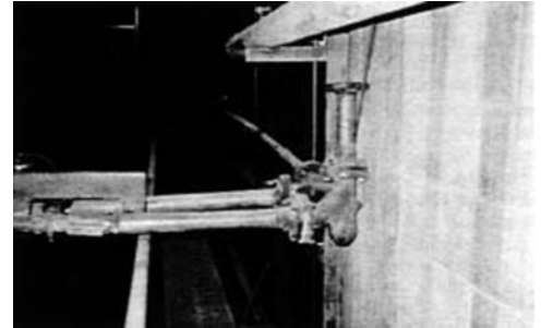
The solution to conveying system elbow wear at North Incinerator: Smart Elbow® deflection elbow in use in the lime injection conveying system.
