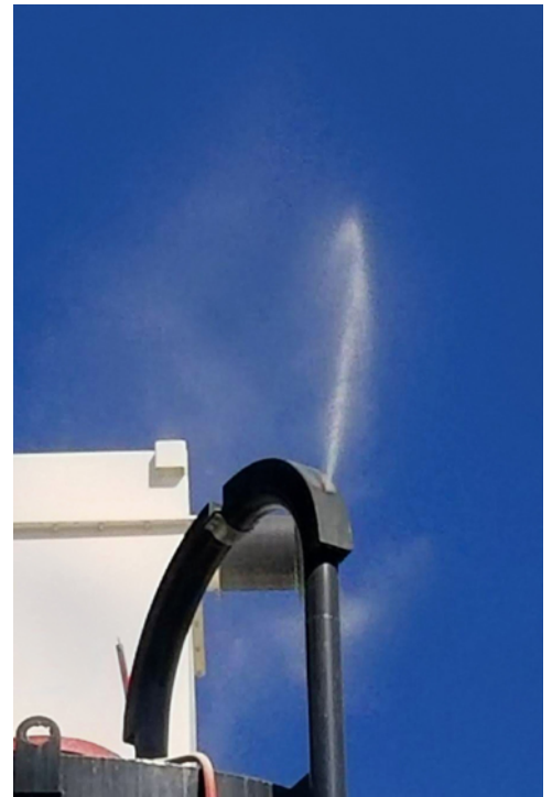
Abrasive silica sand for pavement products conveyed at 1000 cfm (0.47 cu m/sec) through steel pipes was blowing out long sweep elbows and reinforced elbows at Sealmaster, Allentown, PA.
